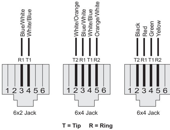
Figure B-3. RJ-11 Pinouts
